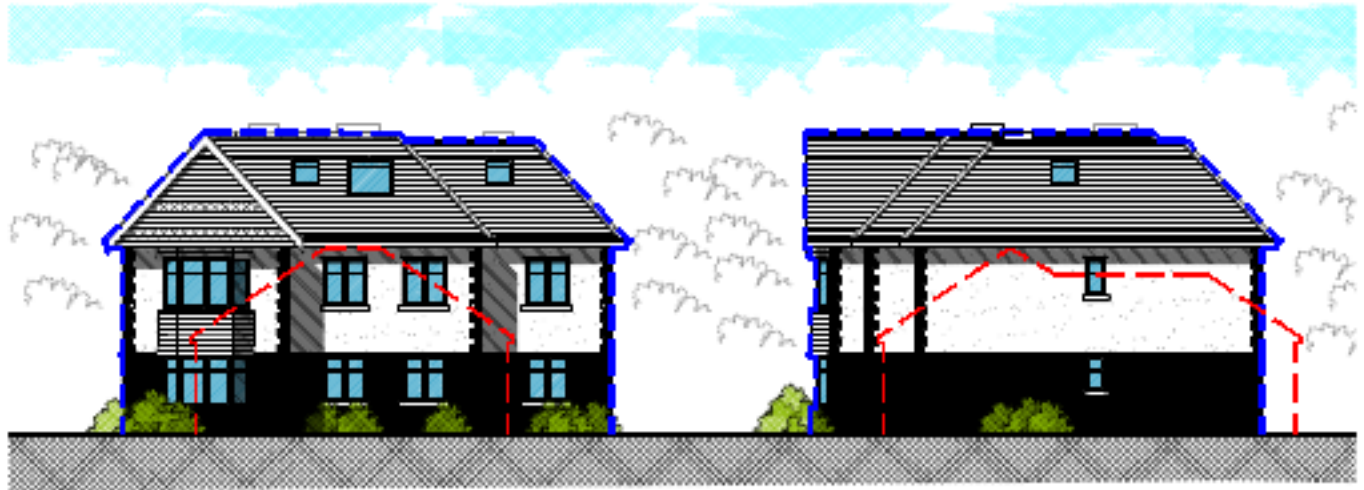
SOUTH ELEVATION 1:100
