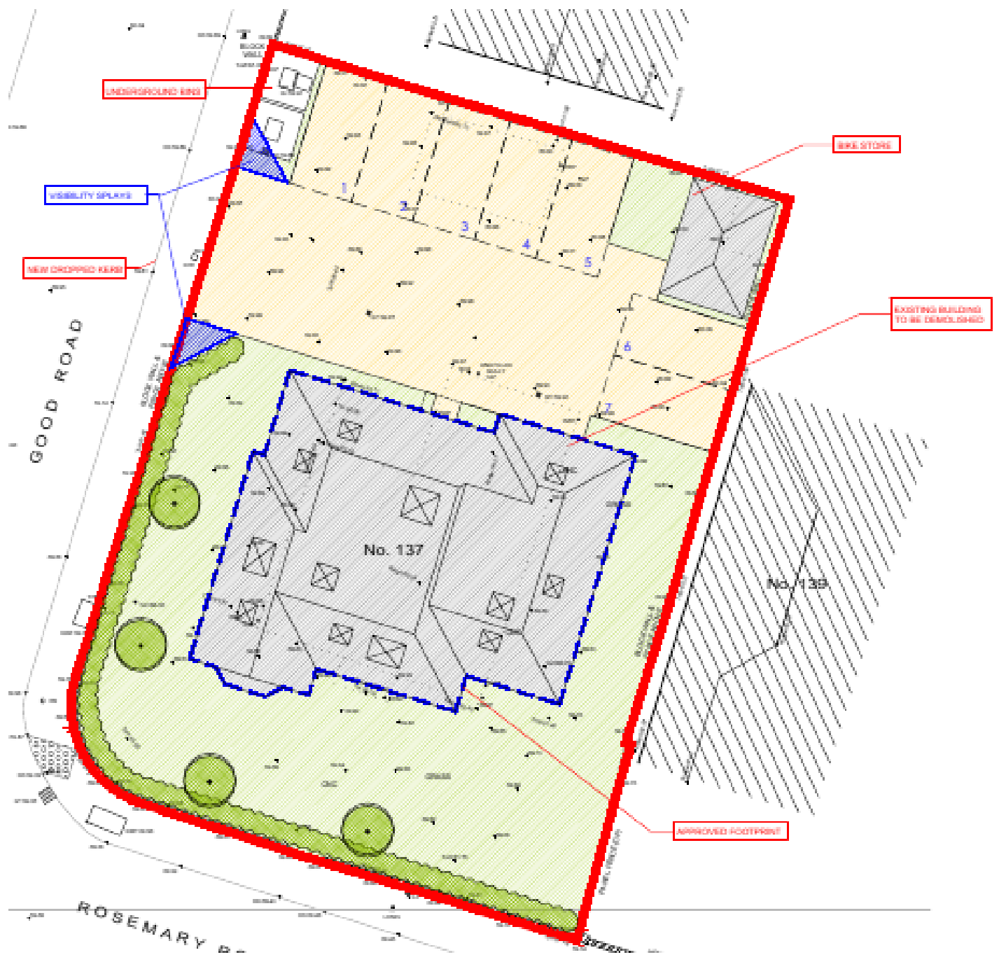
SITE PLAN
